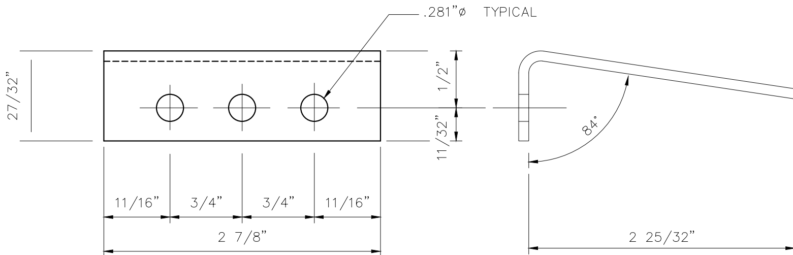
A-34 ATTACHMENT CLIP FOR 4" VERSAWALL PANEL 12 GAGE ASTM-653 GRADE 50, G90 GALV. ATTACHED WITH 1/4"-14 X 4" SS HEX HEAD FASTENERS (2 FASTENERS PER CLIP)
